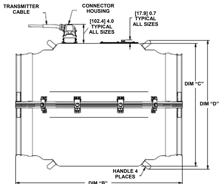
Side View Typical of 17" Through 30" Sensor Heads
