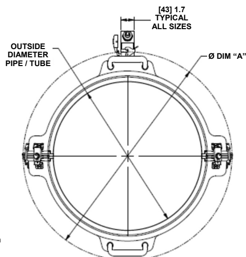
End View Typical of 410mm Through 758mm Sensor Heads
