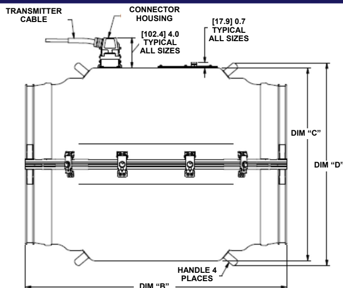
Side View Typical of 10" Through 16" & Metric Equivalent Sensor Heads
