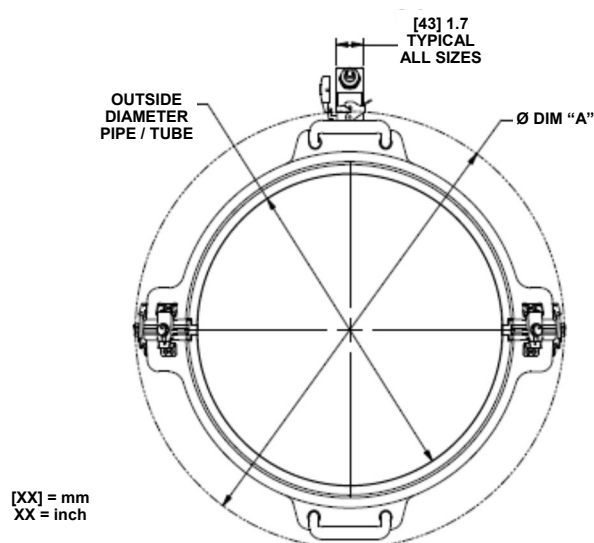
End View Typical of 10" Through 16" & Metric Equivalent Sensor Heads
